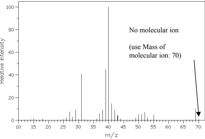
Mass Spec
