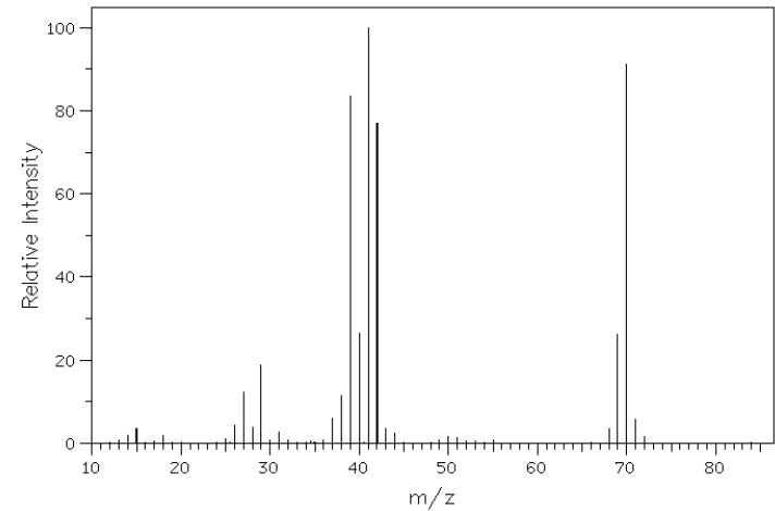
Mass Spec
