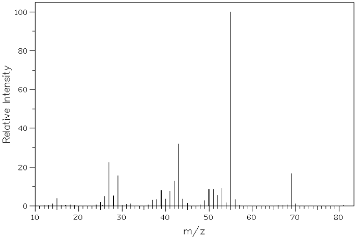
Mass Spec
