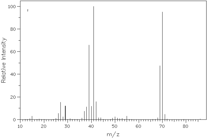
Mass Spec
